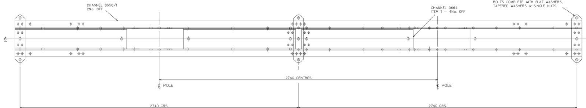
PLAN
